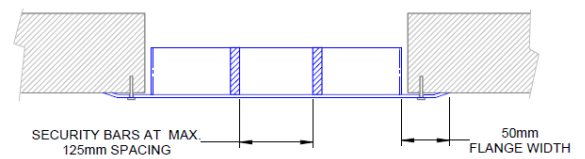
MAXIMUM SECURITY PERFORATED AIR GRILLE SE-MSP-R (REAR FIX)
